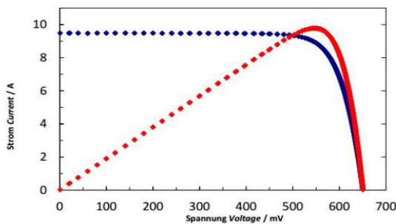
IV curve
